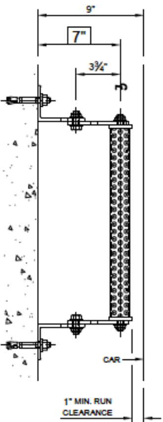
6 PIT LADDER PLAN SCALE: 1-1/2"=1'-0" POSITION: RUNG Ⓞ 7"
